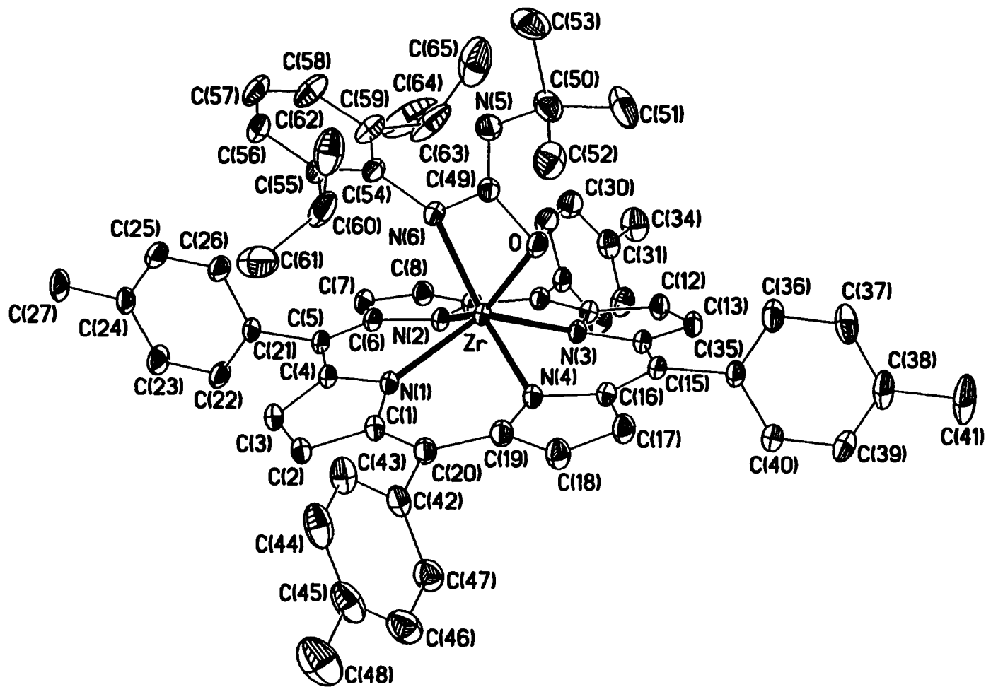
Figure 3. ORTEP representation of (TTP)Zr( \eta^2 -NAr T C(=N T Bu)O). Thermal ellipsoids drawn at 30% probability level.
