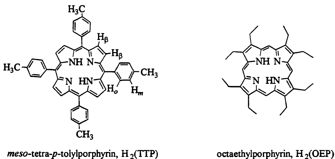
Figure 1. Common synthetic porphyrins.
