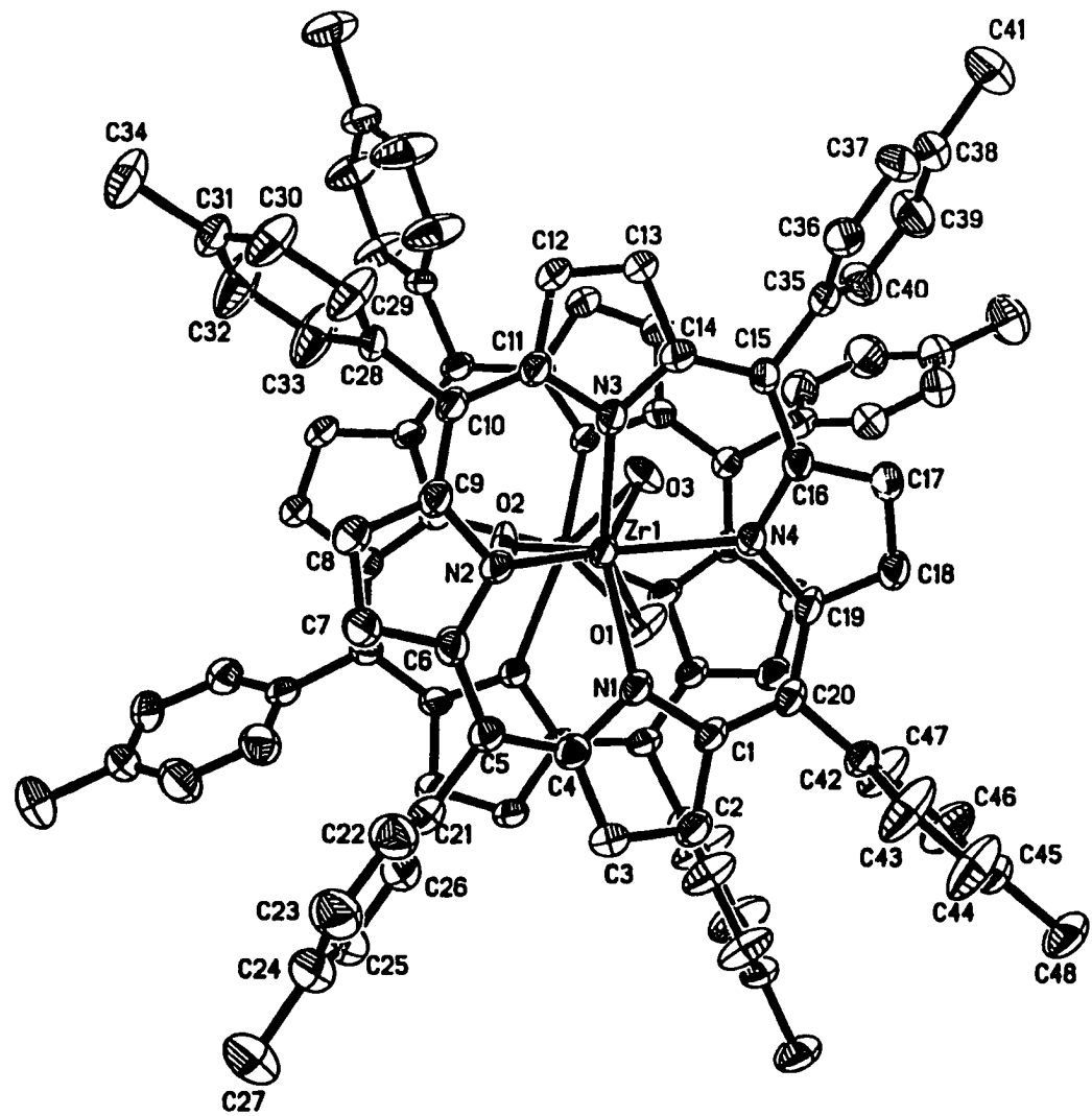
Figure 5. Top view of complex 5, [(\text{TTP})\text{Zr}]_2(\mu\text{-O})(\mu\text{-OH})_2 . Thermal ellipsoids are drawn at the 50% probability level.
