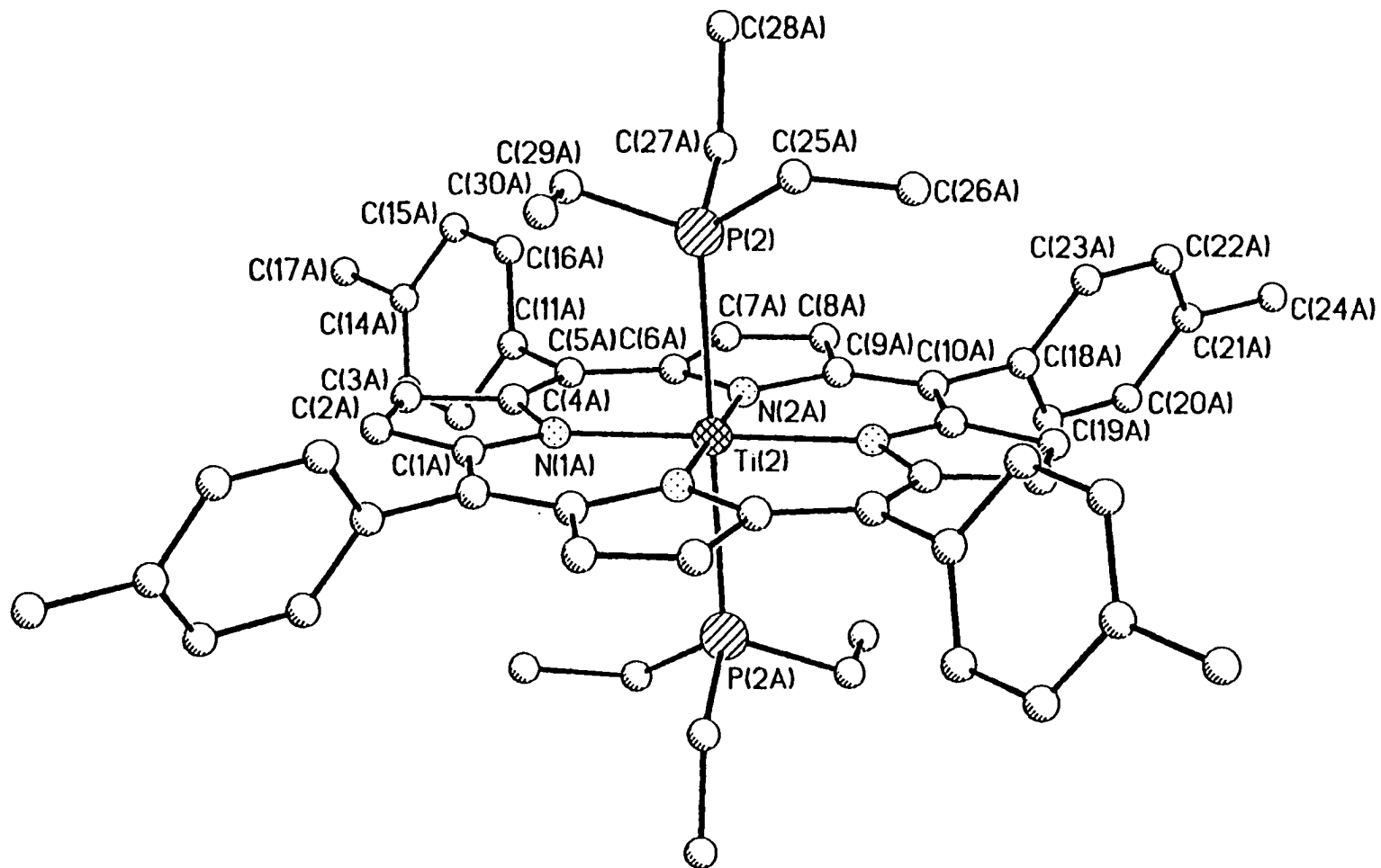
Figure 1. Ball and stick representation of (TTP)Ti(PEt_3)_2 .
