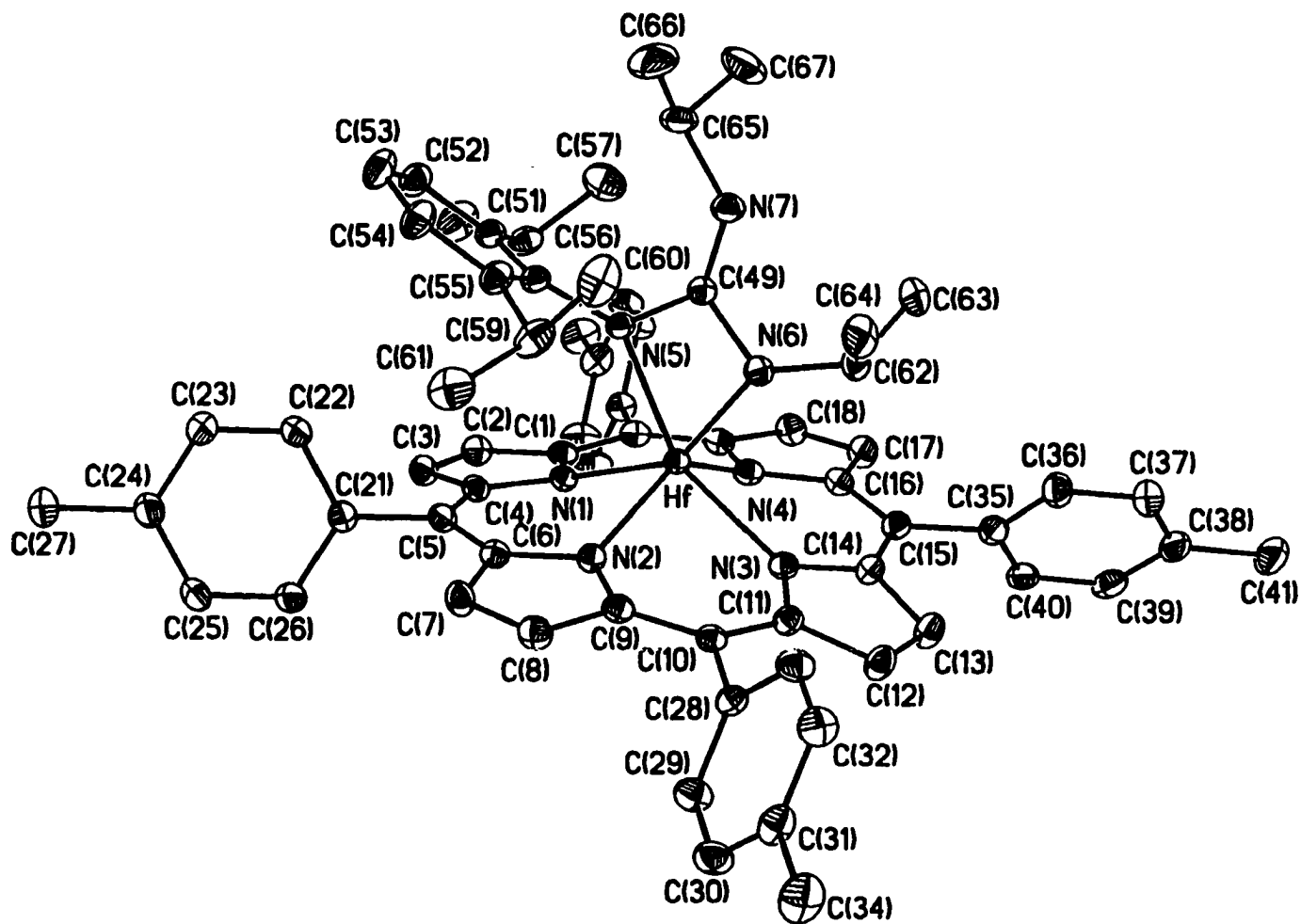
Figure 5. ORTEP representation of (TTP)Hf(\eta^2-NAr^{Pr}C(=N^{Pr})N^{Pr}) . Thermal ellipsoids drawn at 30% probability level.
