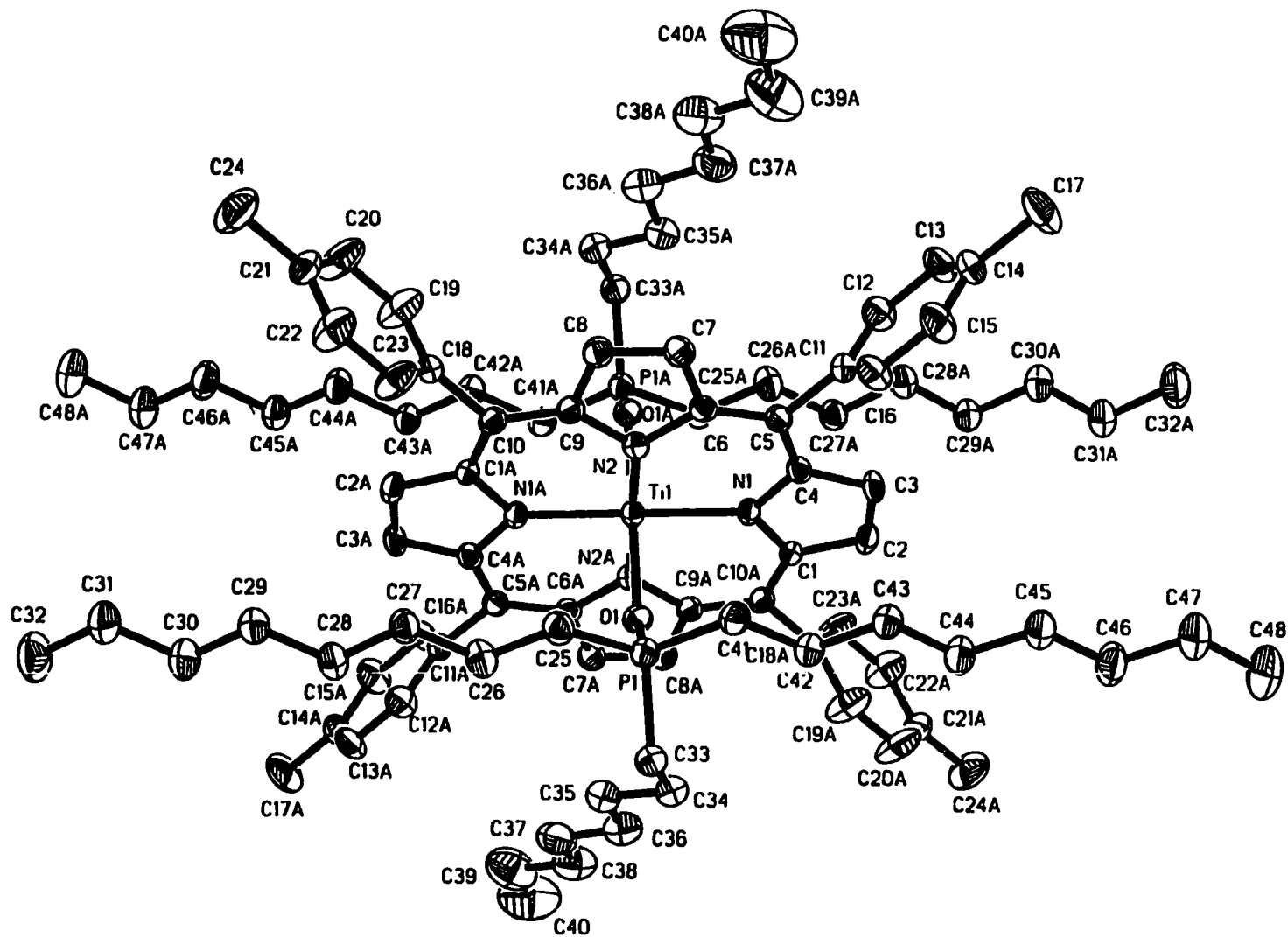
Figure 1. ORTEP representation of (\text{TTP})\text{Ti}(\text{OPOct})_2 . Thermal ellipsoids drawn at the 50% probability level.
