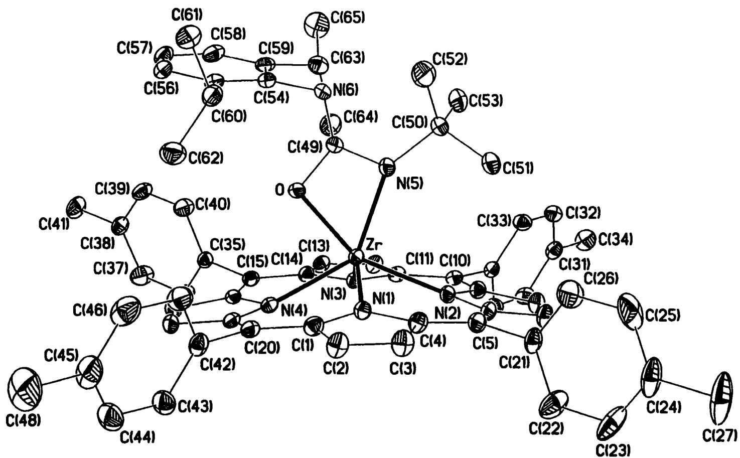
Figure 4. ORTEP representation of (TTP)Zr(η 2 -N i BuC(=NAr T )O). Thermal ellipsoids drawn at 30% probability level.
