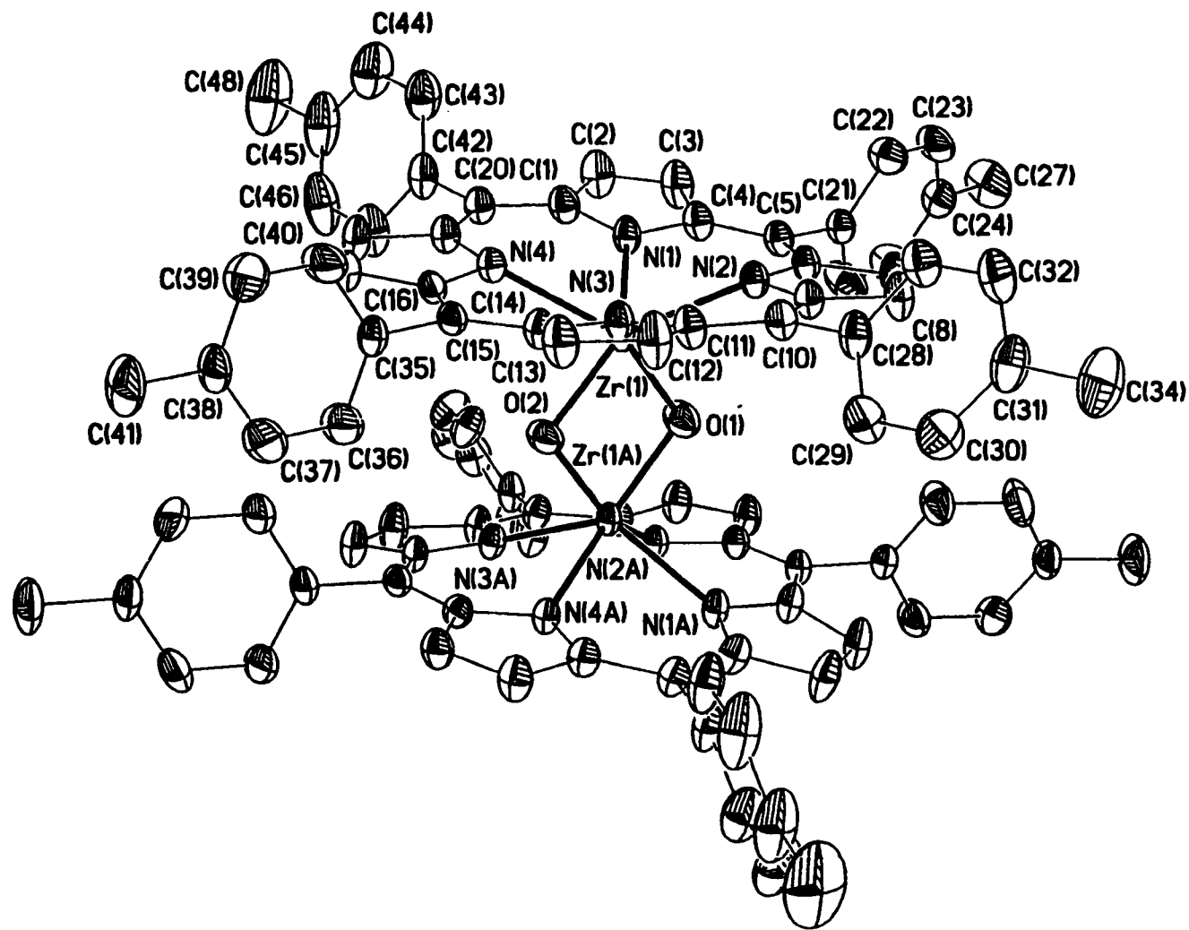
Figure 4. Molecular structure of [(TTP)ZrO]_2 (4). Thermal ellipsoids are drawn at the 30% probability level.
